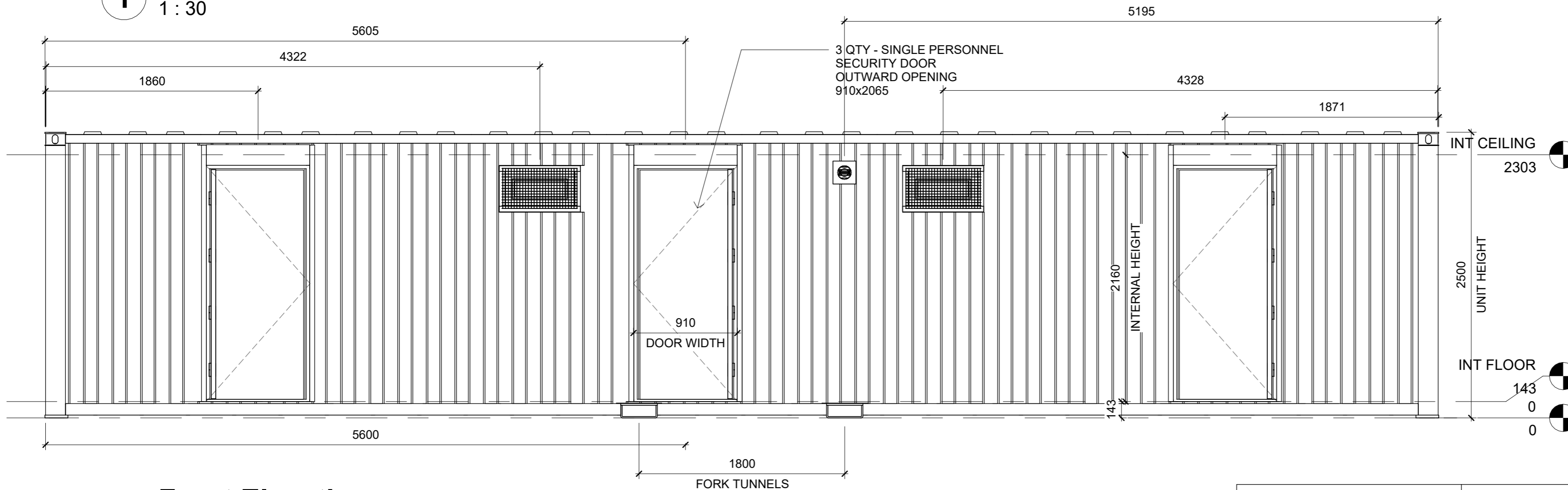
3 Front Elevation 1 : 30
