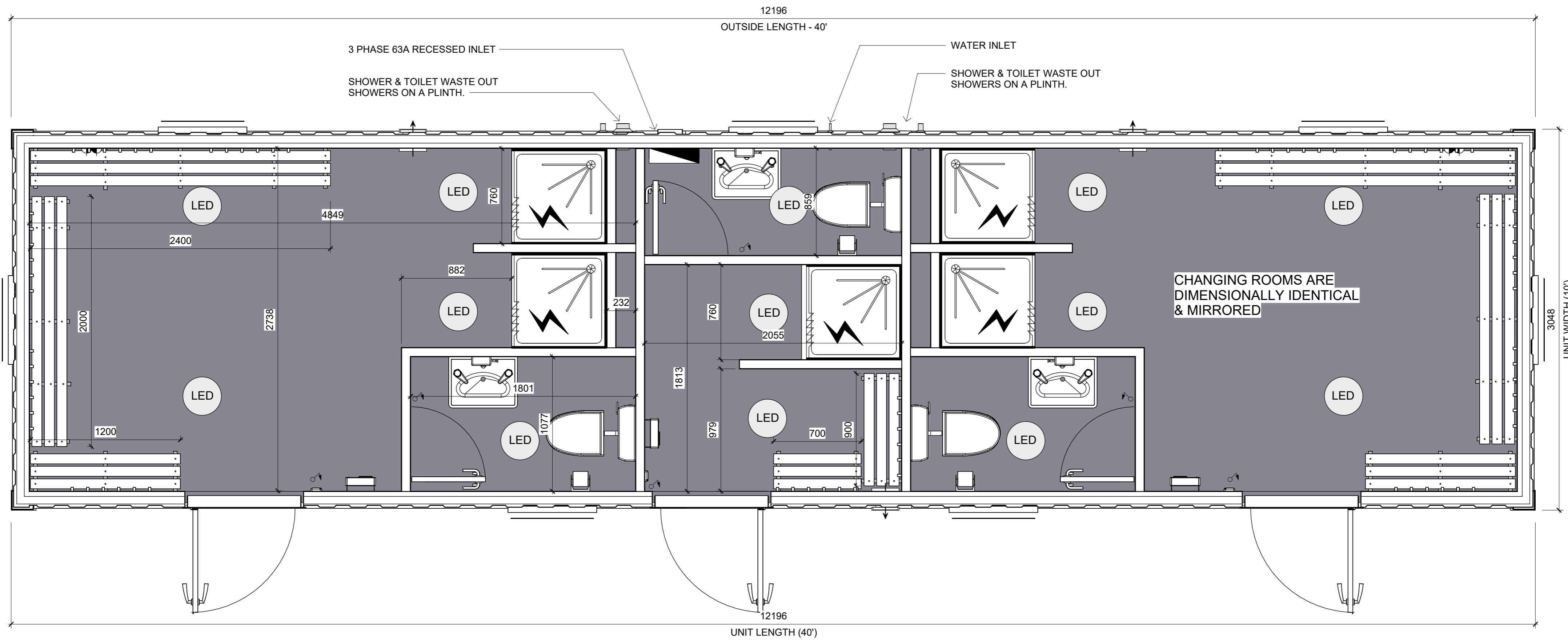
1 Plan View Lining 1 : 22
