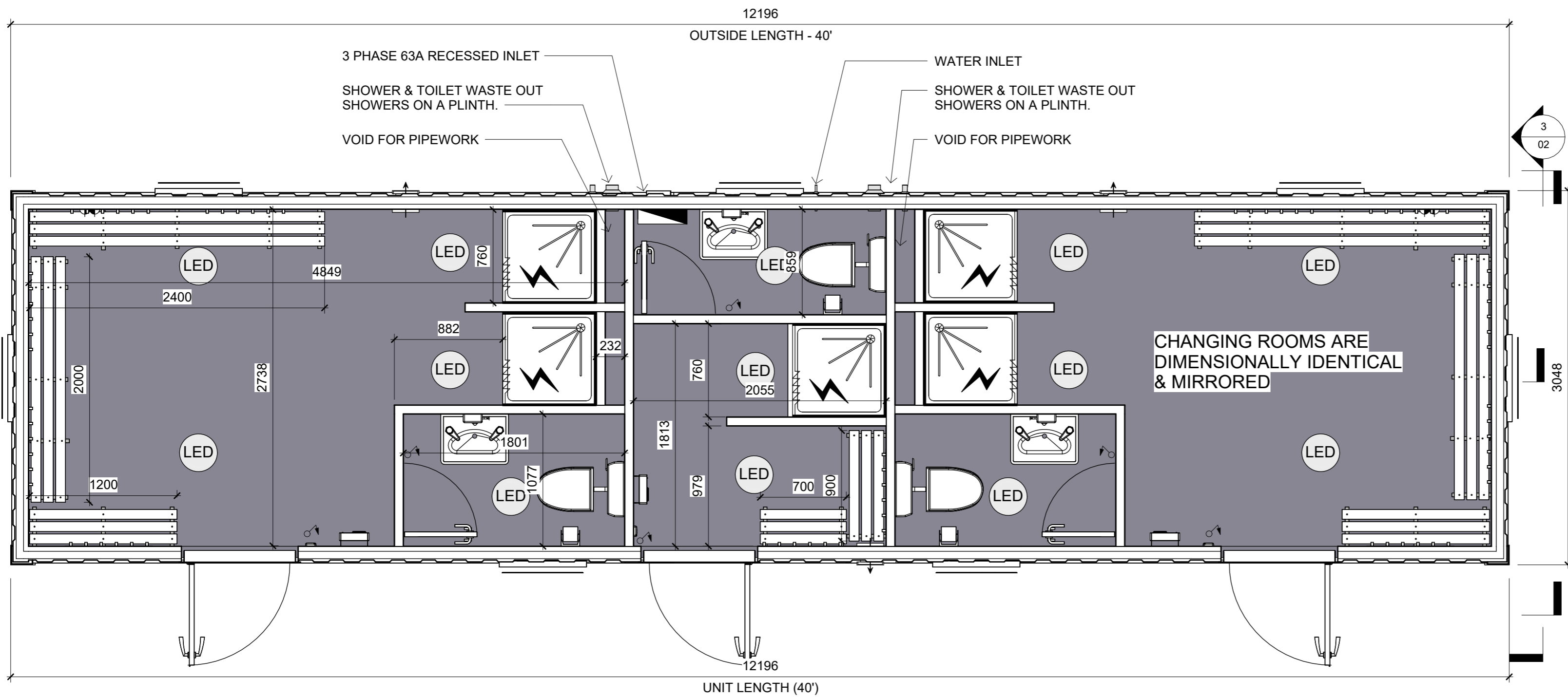
1 Plan View 1 : 30
